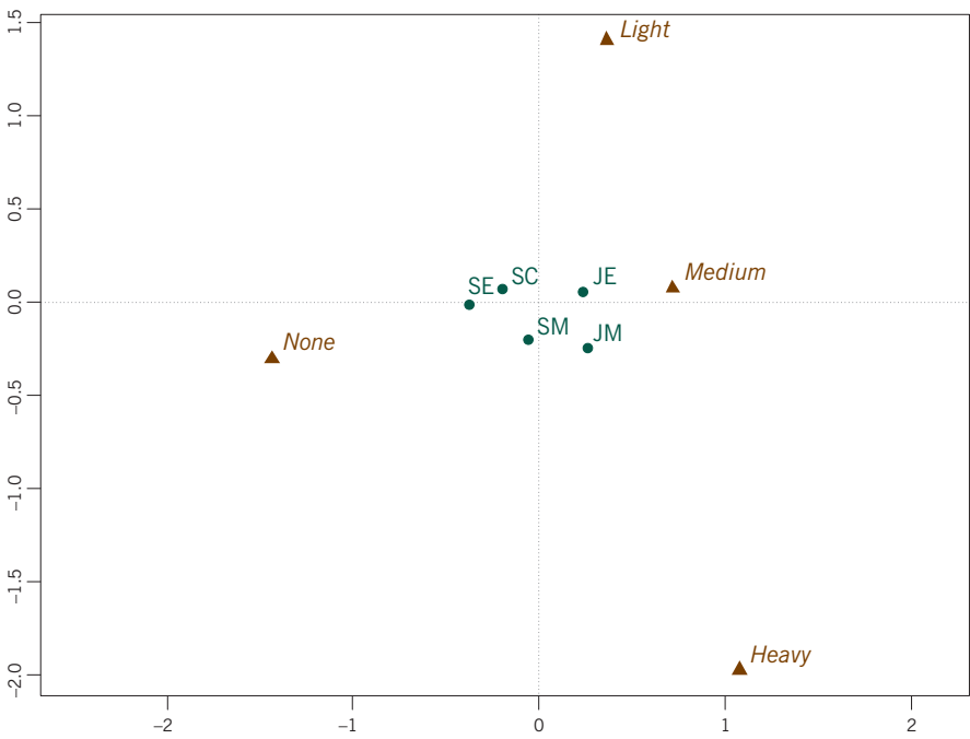
Exhibit 8.2: Row asymmetric CA map (i.e., row principal biplot) of the “smoking” data, with rows in principal coordinates and columns in standard coordinates. This map is reproduced directly from the ca package in R —see the Computational Appendix
